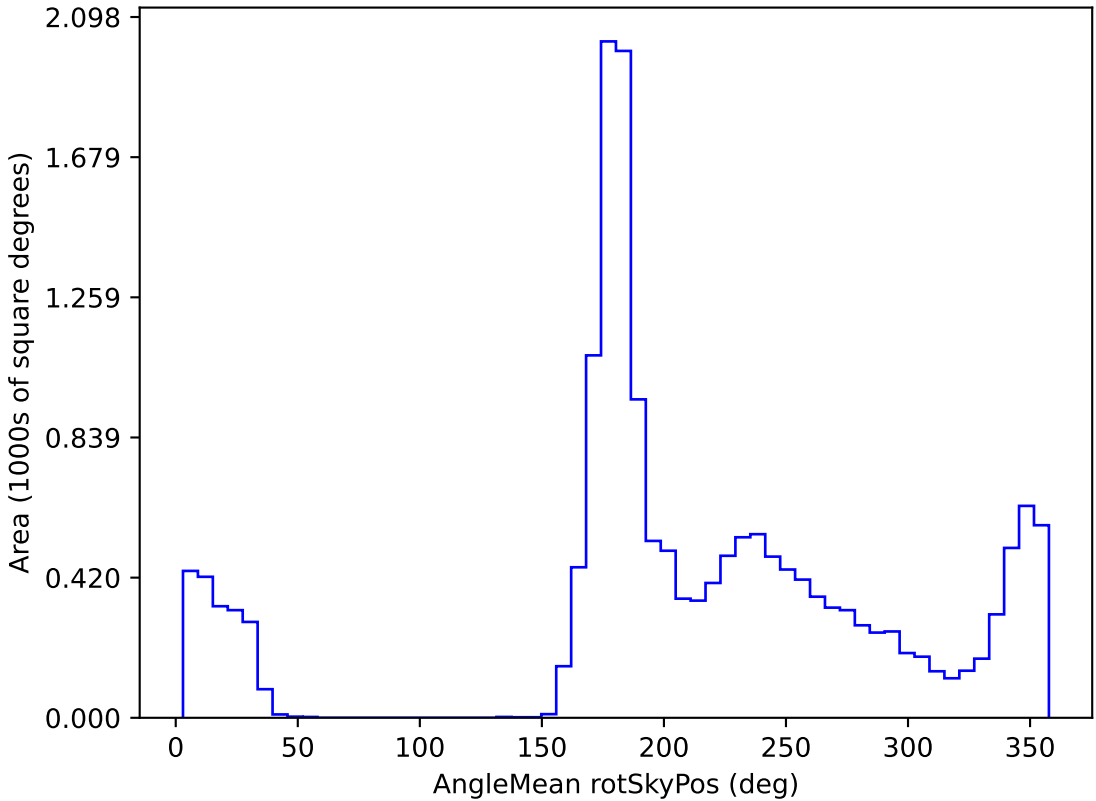
too_elab_r8_d2_griz_v3.4_10yrs WFD r band: AngleMean rotSkyPos
