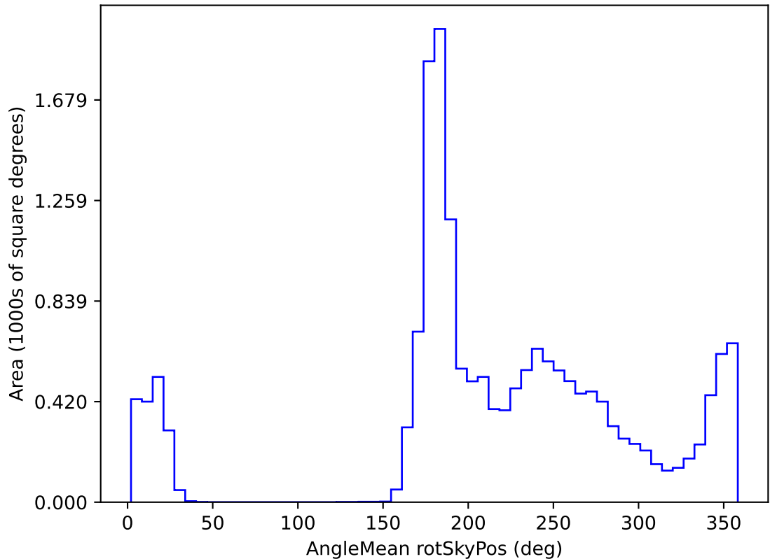
too_elab_r8_d2_griz_v3.4_10yrs WFD i band: AngleMean rotSkyPos
