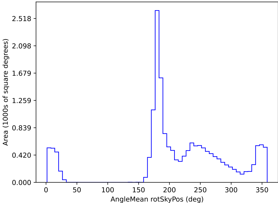
too_elab_r8_d2_griz_v3.4_10yrs WFD all bands: AngleMean rotSkyPos
