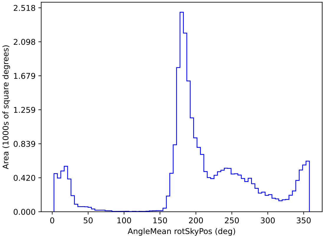
too_elab_r8_d2_griz_v3.4_10yrs All sky i band: AngleMean rotSkyPos
