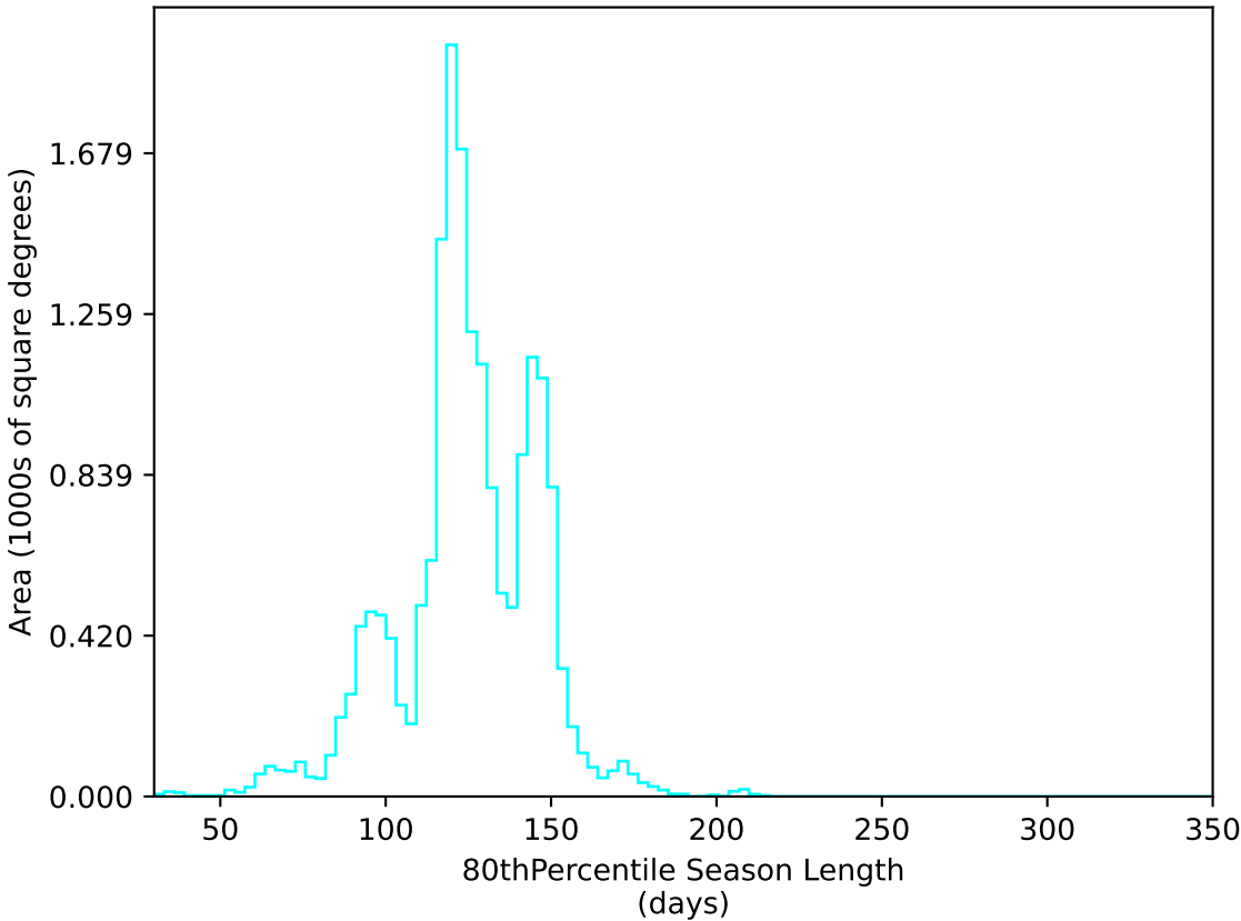
too_elab_r8_d2_griz_v3.4_10yrs WFD u band: 80thPercentile Season Length
