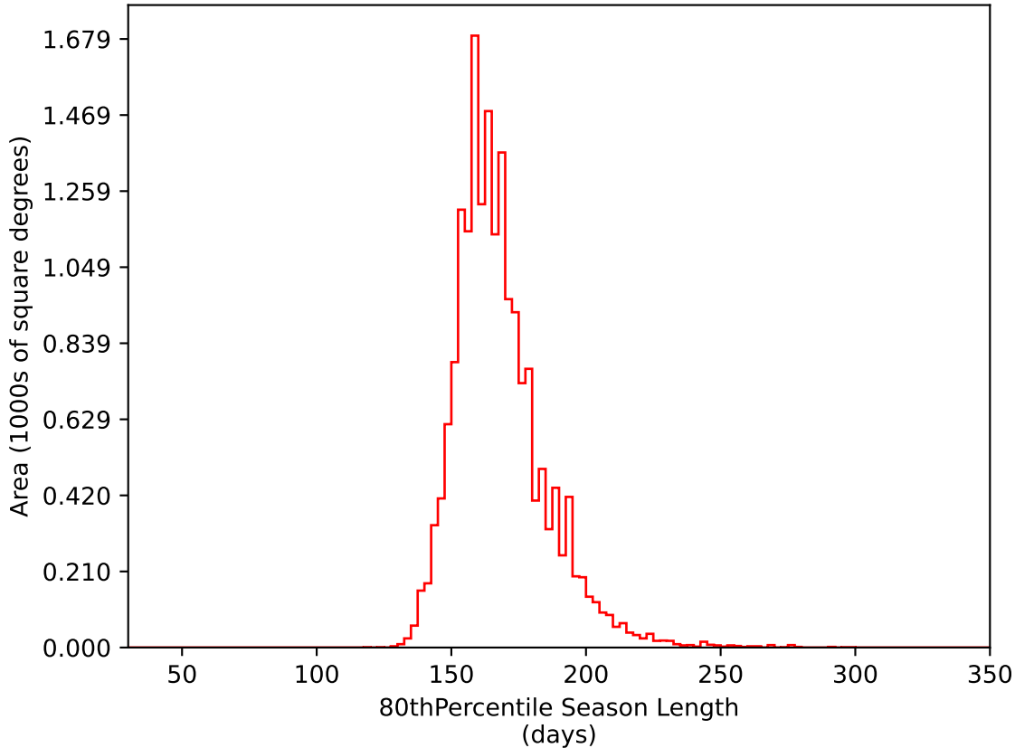
too_elab_r8_d2_griz_v3.4_10yrs WFD i band: 80thPercentile Season Length
