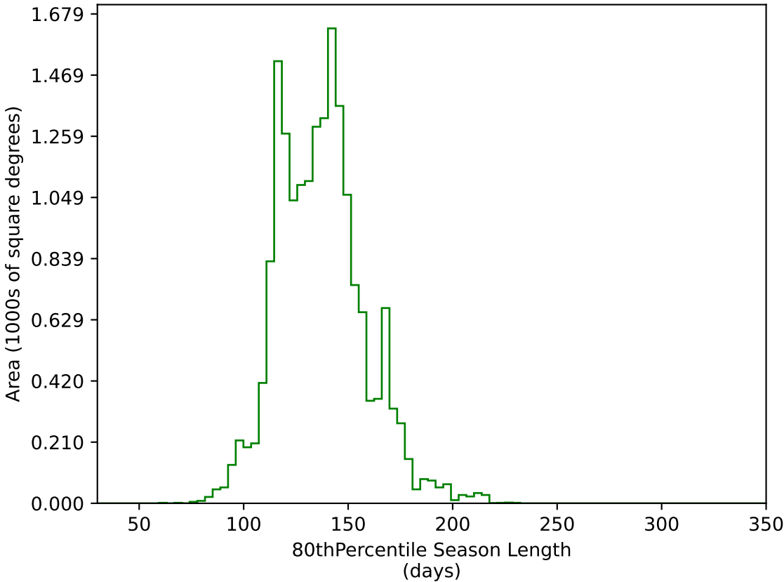
too_elab_r8_d2_griz_v3.4_10yrs WFD g band: 80thPercentile Season Length
