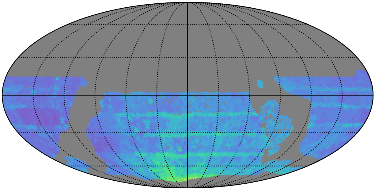
too_elab_r8_d2_griz_v3.4_10yrs WFD all bands: 80thPercentile Season Length
