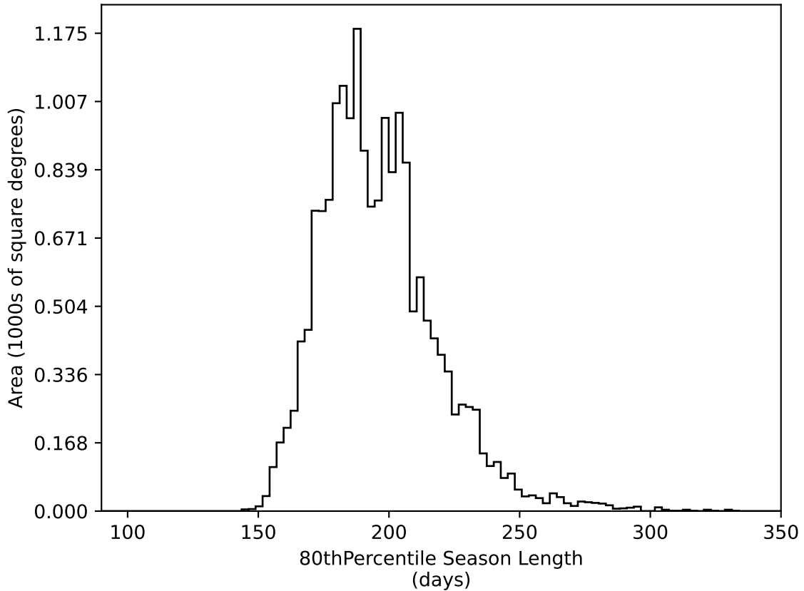
too_elab_r8_d2_griz_v3.4_10yrs WFD all bands: 80thPercentile Season Length
