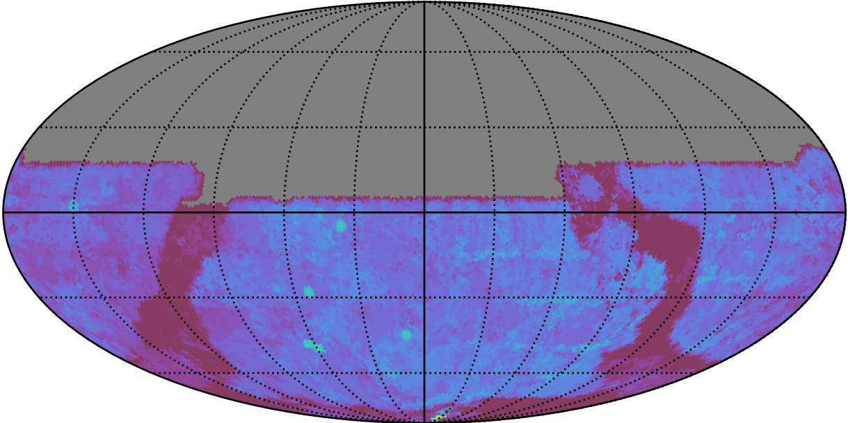
too_elab_r8_d2_griz_v3.4_10yrs All sky u band: 80thPercentile Season Length
