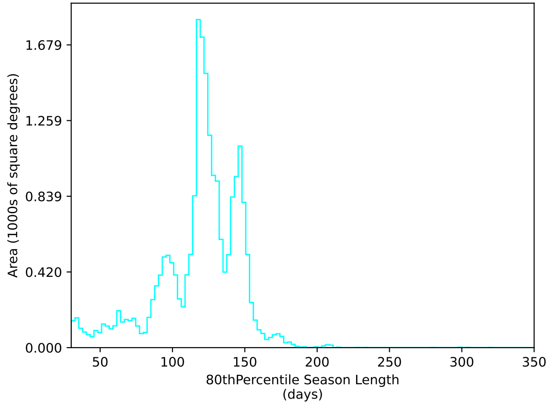
too_elab_r8_d2_griz_v3.4_10yrs All sky u band: 80thPercentile Season Length
