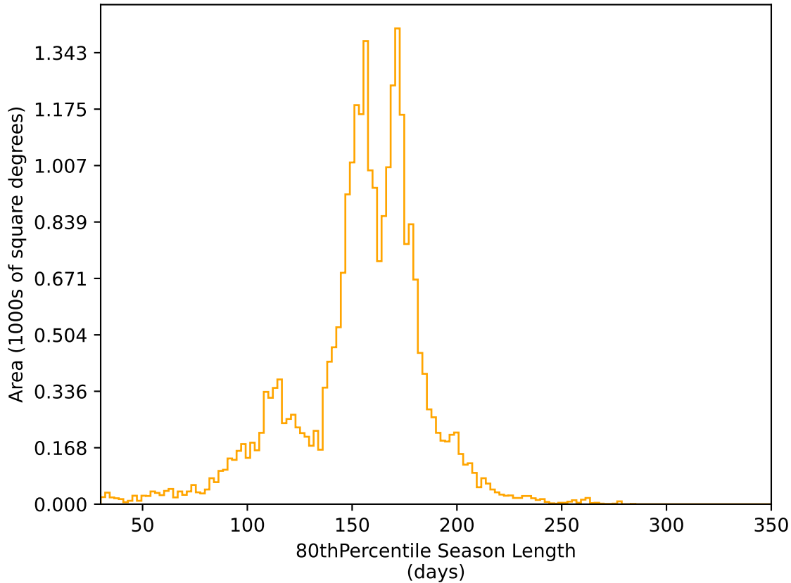
too_elab_r8_d2_griz_v3.4_10yrs All sky r band: 80thPercentile Season Length
