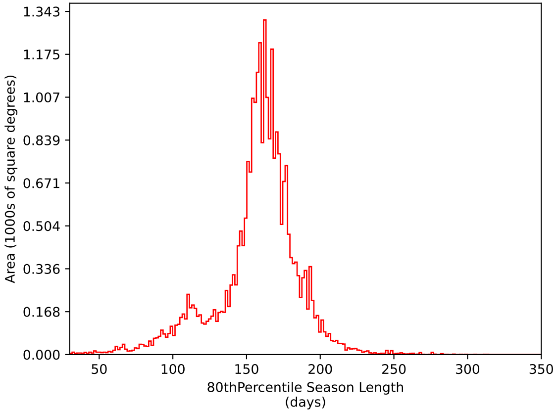
too_elab_r8_d2_griz_v3.4_10yrs All sky i band: 80thPercentile Season Length
