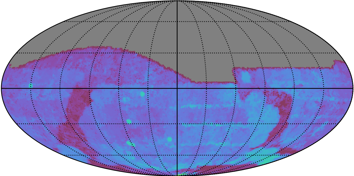
too_elab_r8_d2_griz_v3.4_10yrs All sky g band: 80thPercentile Season Length
