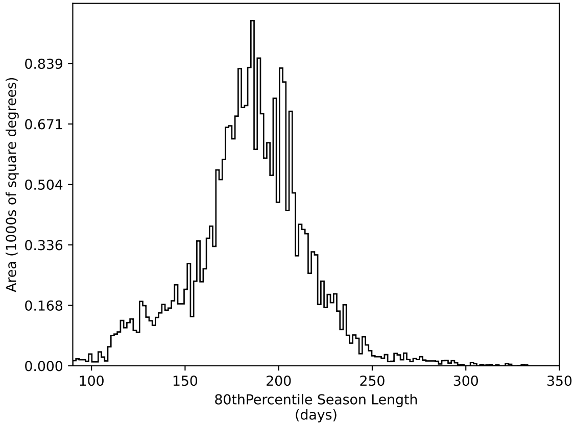
too_elab_r8_d2_griz_v3.4_10yrs All sky all bands: 80thPercentile Season Length
