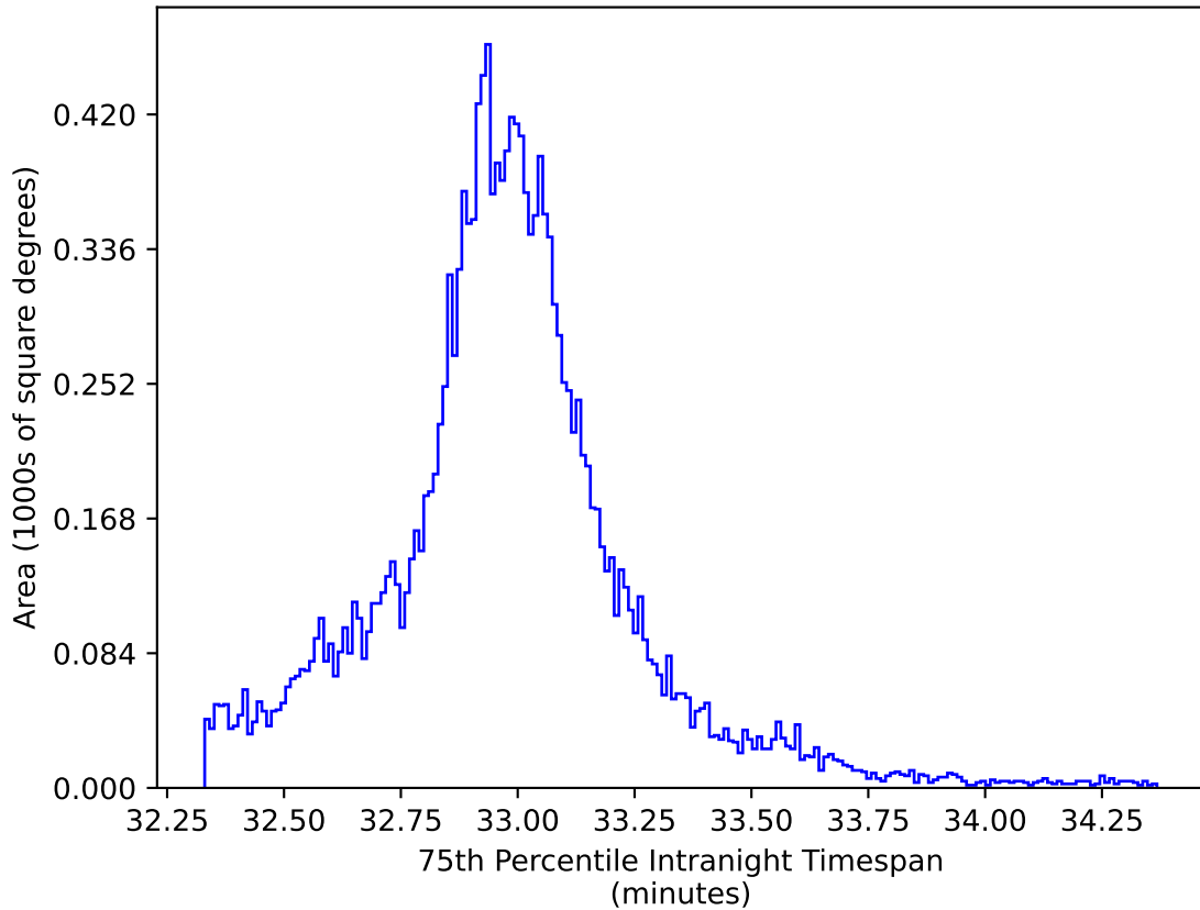
too_elab_r8_d2_griz_v3.4_10yrs WFD y band: 75th Percentile Intranight Timespan
