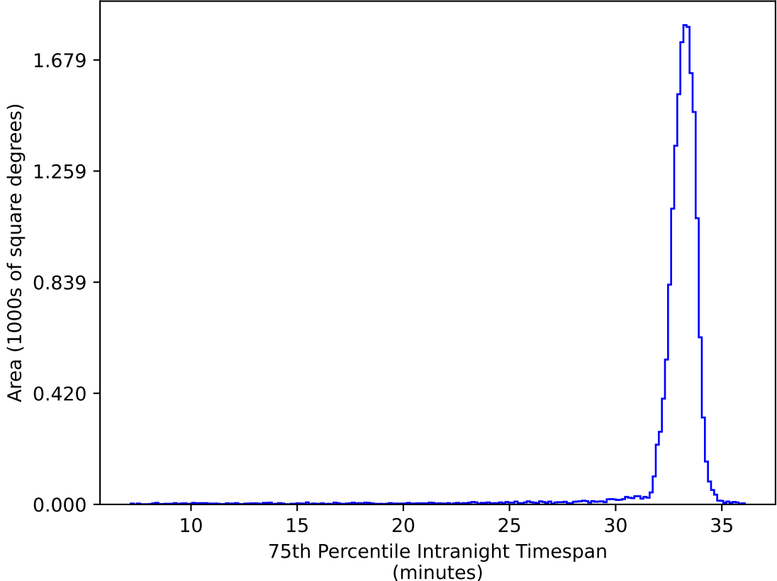
too_elab_r8_d2_griz_v3.4_10yrs WFD ug bands: 75th Percentile Intranight Timespan
