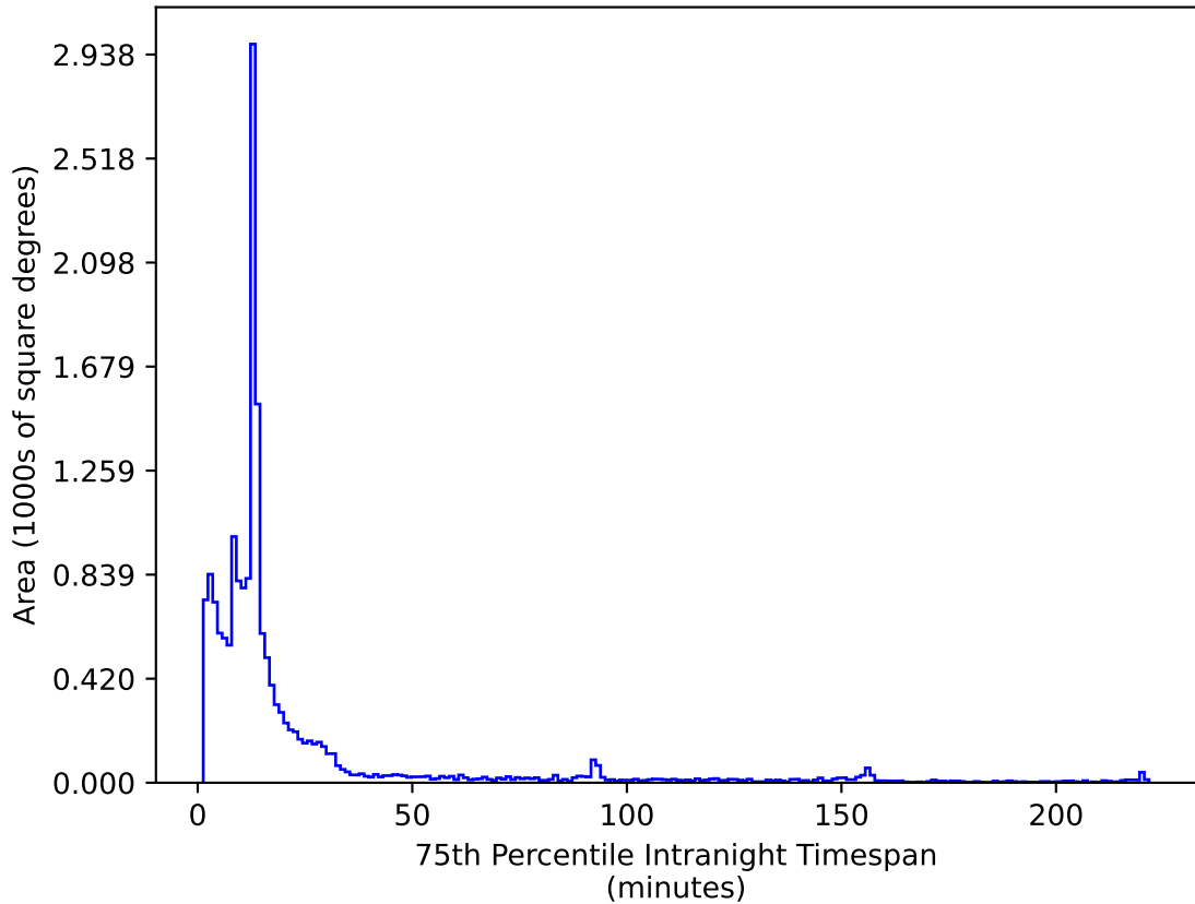
too_elab_r8_d2_griz_v3.4_10yrs WFD i band: 75th Percentile Intranight Timespan
