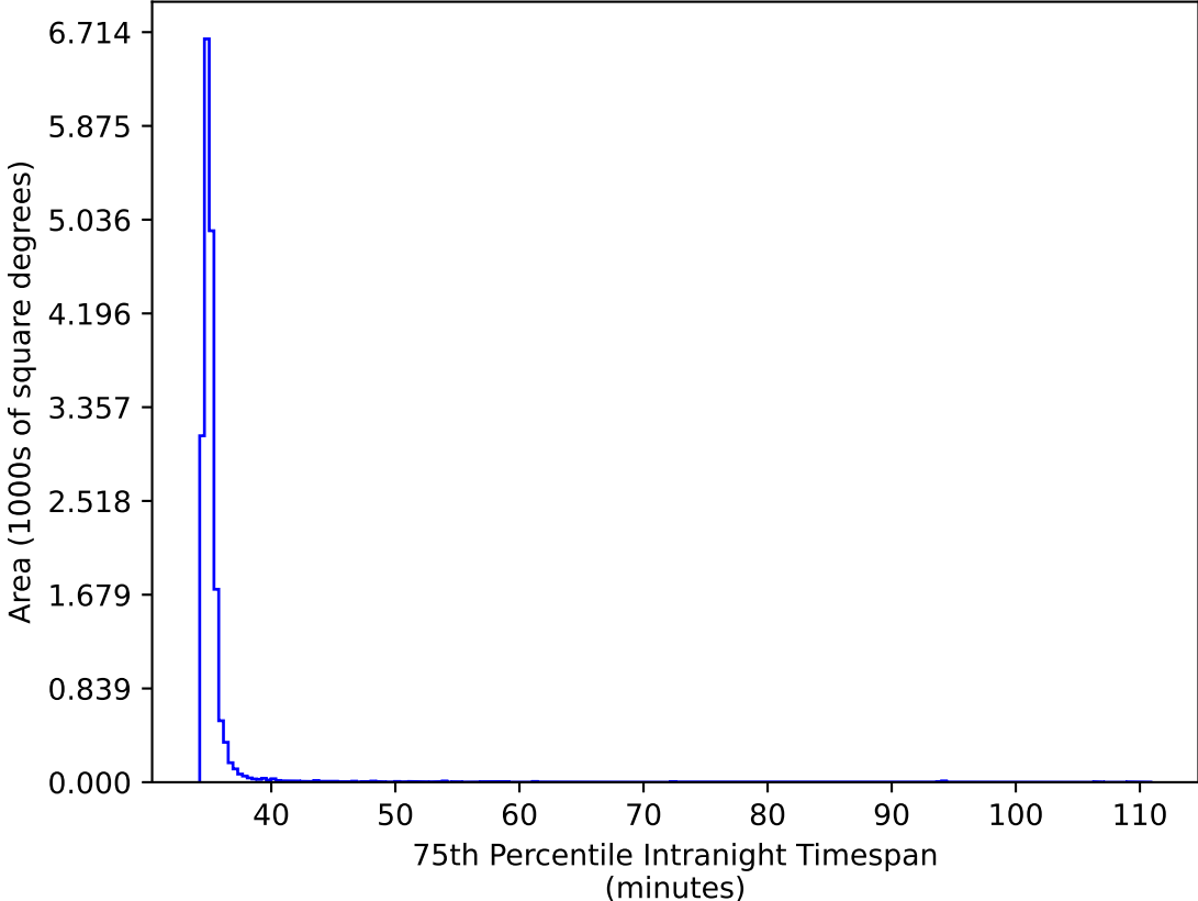
too_elab_r8_d2_griz_v3.4_10yrs WFD gr bands: 75th Percentile Intranight Timespan
