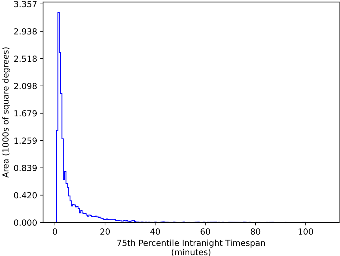
too_elab_r8_d2_griz_v3.4_10yrs WFD g band: 75th Percentile Intranight Timespan
