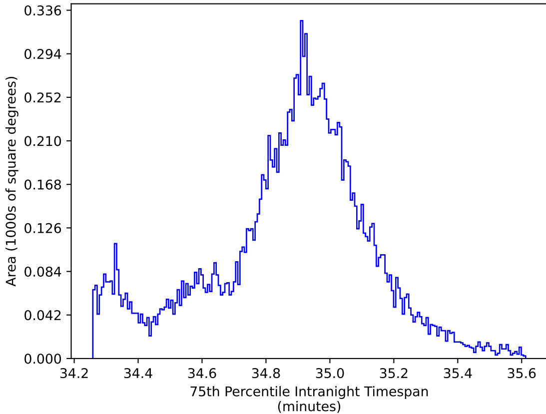
too_elab_r8_d2_griz_v3.4_10yrs WFD all bands: 75th Percentile Intranight Timespan
