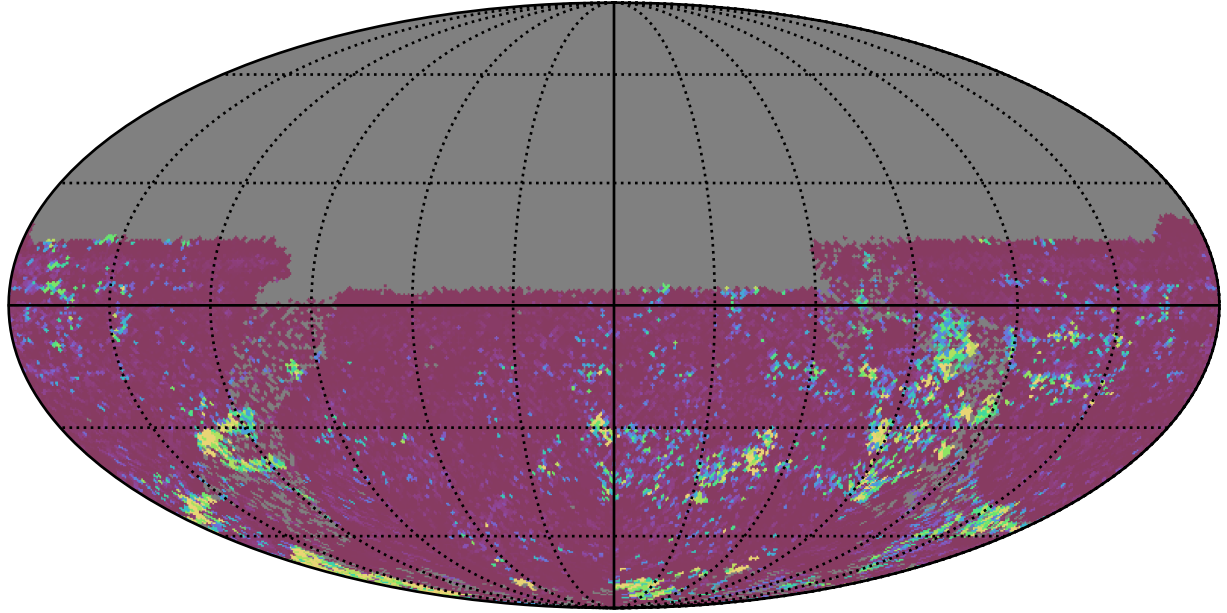
too_elab_r8_d2_griz_v3.4_10yrs All sky u band: 75th Percentile Intranight Timespan
