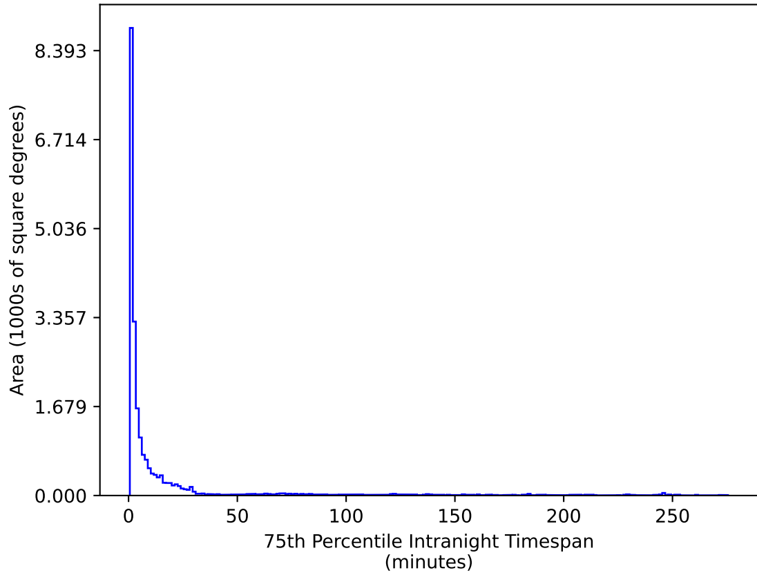
too_elab_r8_d2_griz_v3.4_10yrs All sky u band: 75th Percentile Intranight Timespan
