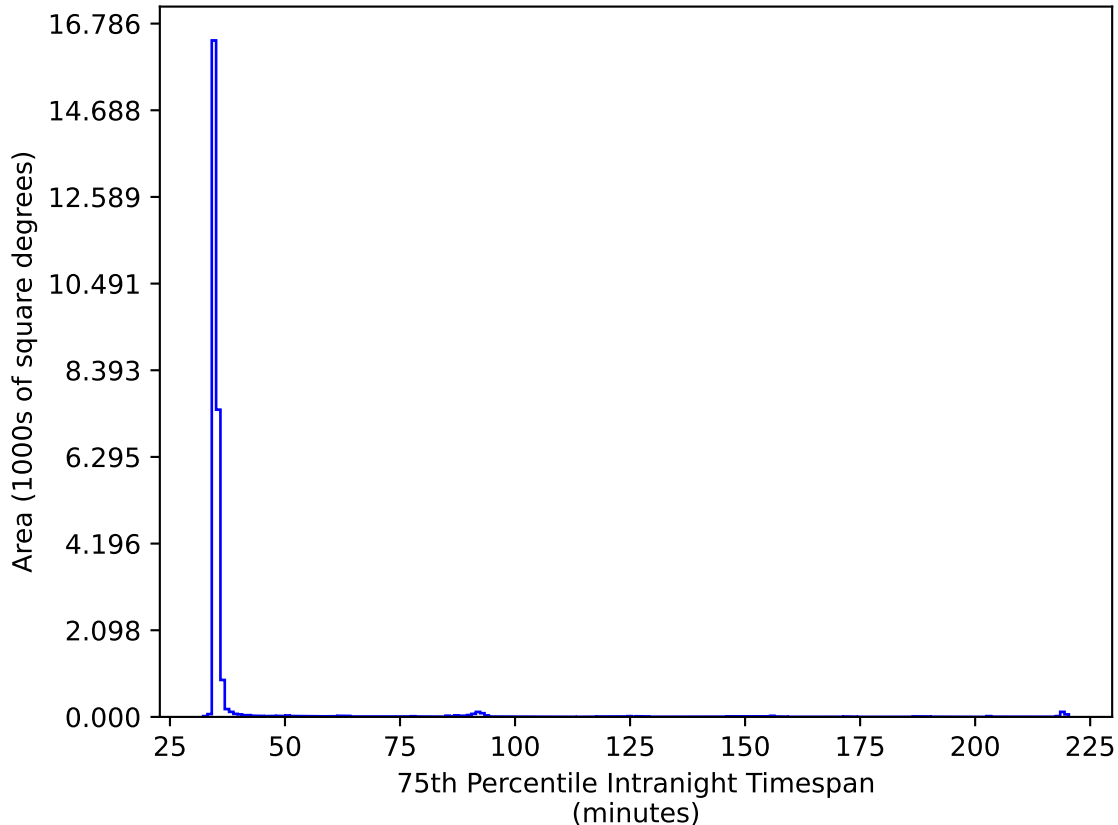
too_elab_r8_d2_griz_v3.4_10yrs All sky ri bands: 75th Percentile Intranight Timespan
