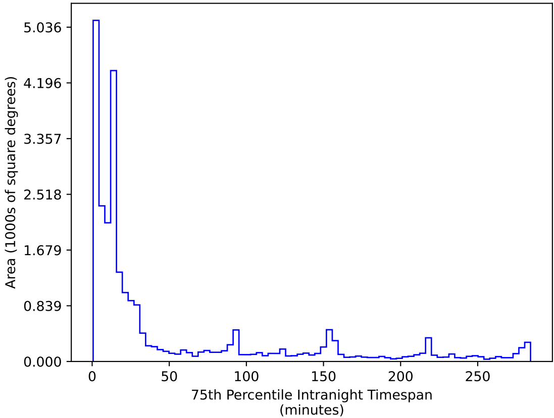
too_elab_r8_d2_griz_v3.4_10yrs All sky r band: 75th Percentile Intranight Timespan
