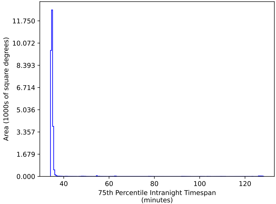
too_elab_r8_d2_griz_v3.4_10yrs All sky iz bands: 75th Percentile Intranight Timespan
