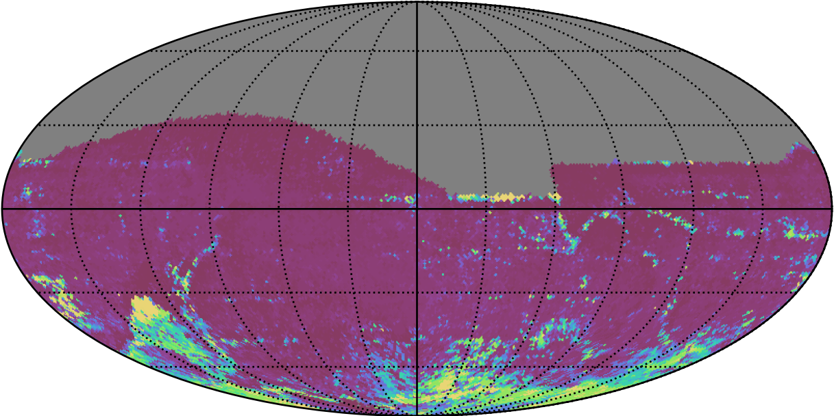
too_elab_r8_d2_griz_v3.4_10yrs All sky i band: 75th Percentile Intranight Timespan
