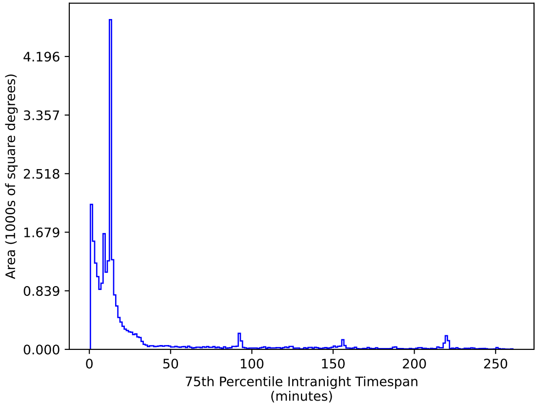
too_elab_r8_d2_griz_v3.4_10yrs All sky i band: 75th Percentile Intranight Timespan
