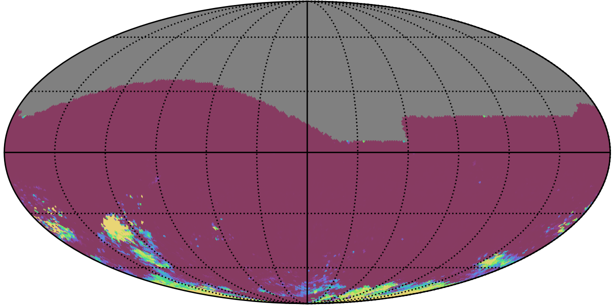
too_elab_r8_d2_griz_v3.4_10yrs All sky gr bands: 75th Percentile Intranight Timespan
