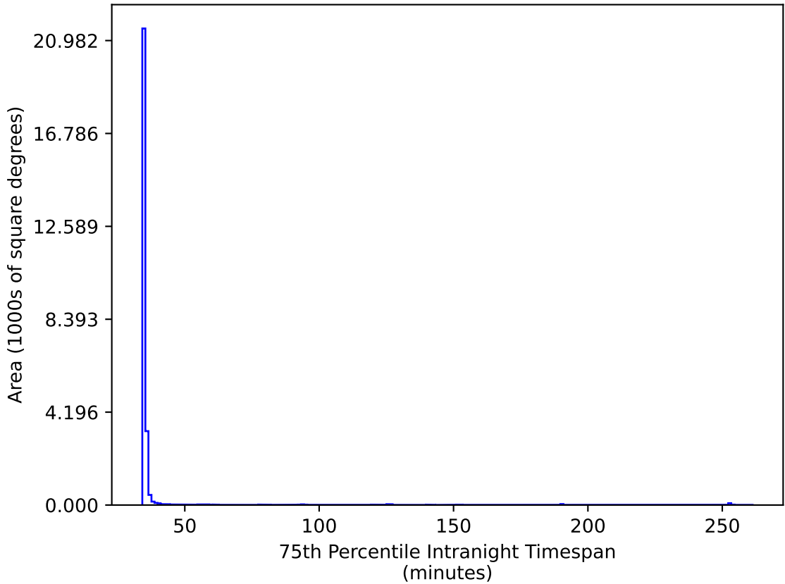
too_elab_r8_d2_griz_v3.4_10yrs All sky gr bands: 75th Percentile Intranight Timespan
