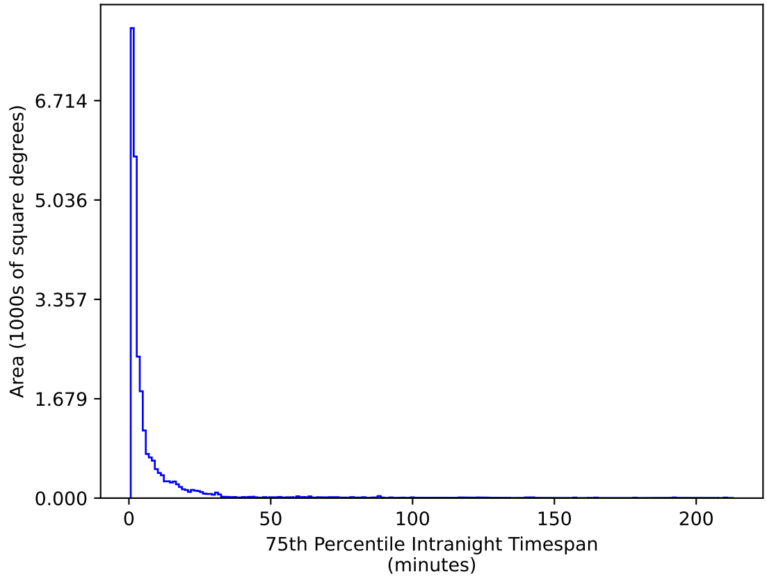
too_elab_r8_d2_griz_v3.4_10yrs All sky g band: 75th Percentile Intranight Timespan
