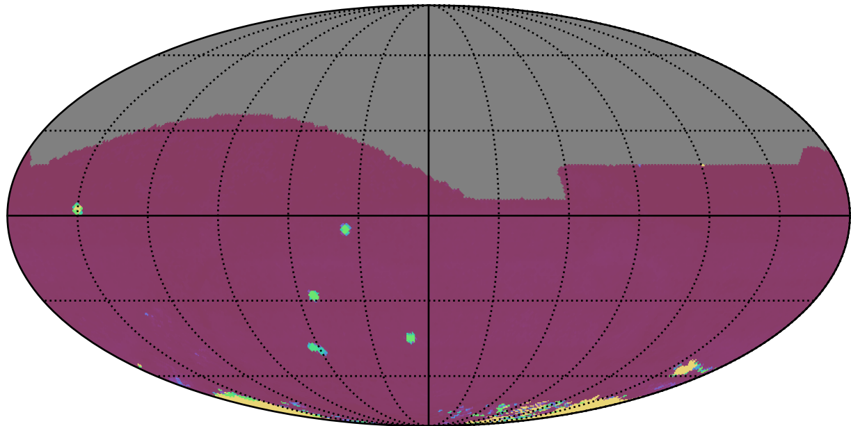
too_elab_r8_d2_griz_v3.4_10yrs All sky all bands: 75th Percentile Intranight Timespan
