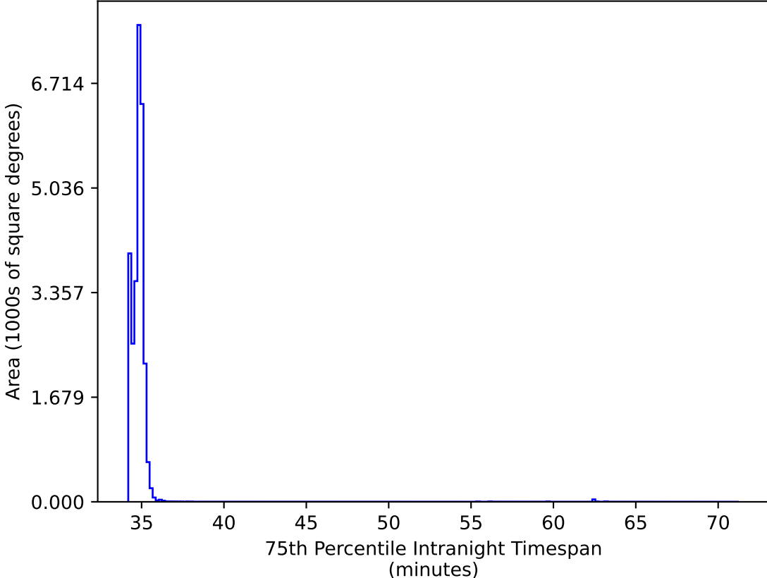
too_elab_r8_d2_griz_v3.4_10yrs All sky all bands: 75th Percentile Intranight Timespan
