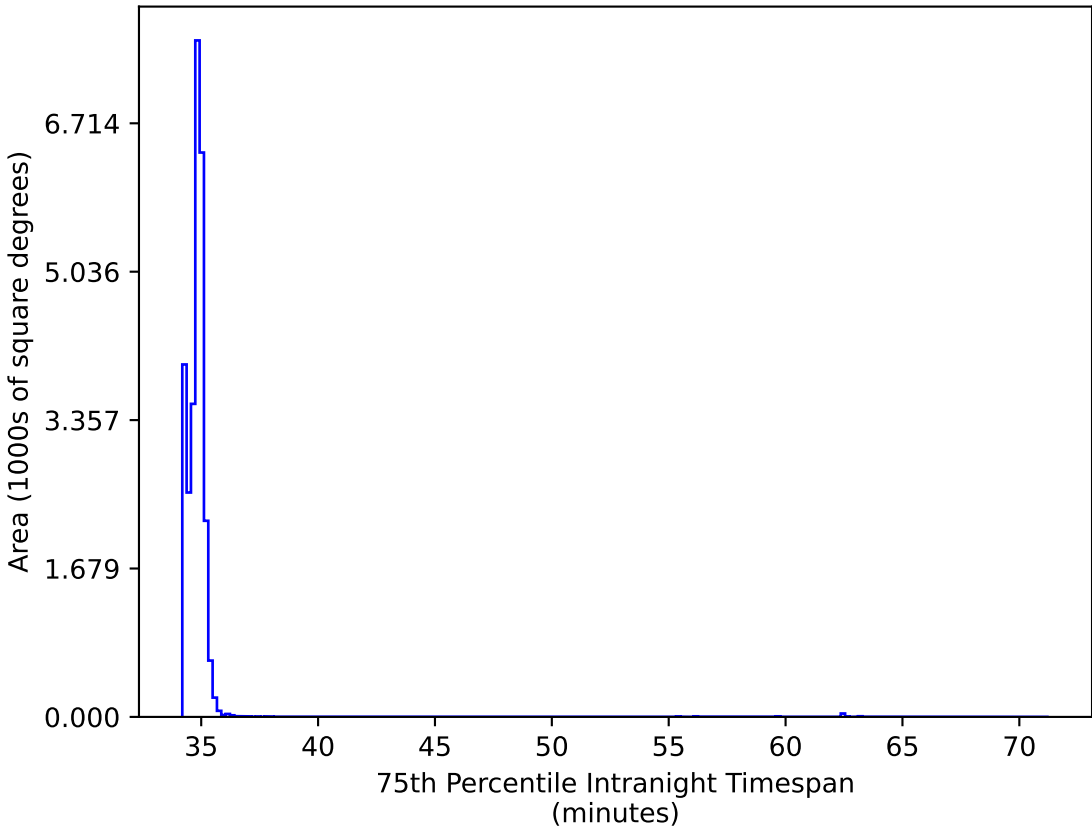
too_elab_r8_d2_griz_v3.4_10yrs All sky: 75th Percentile Intranight Timespan
