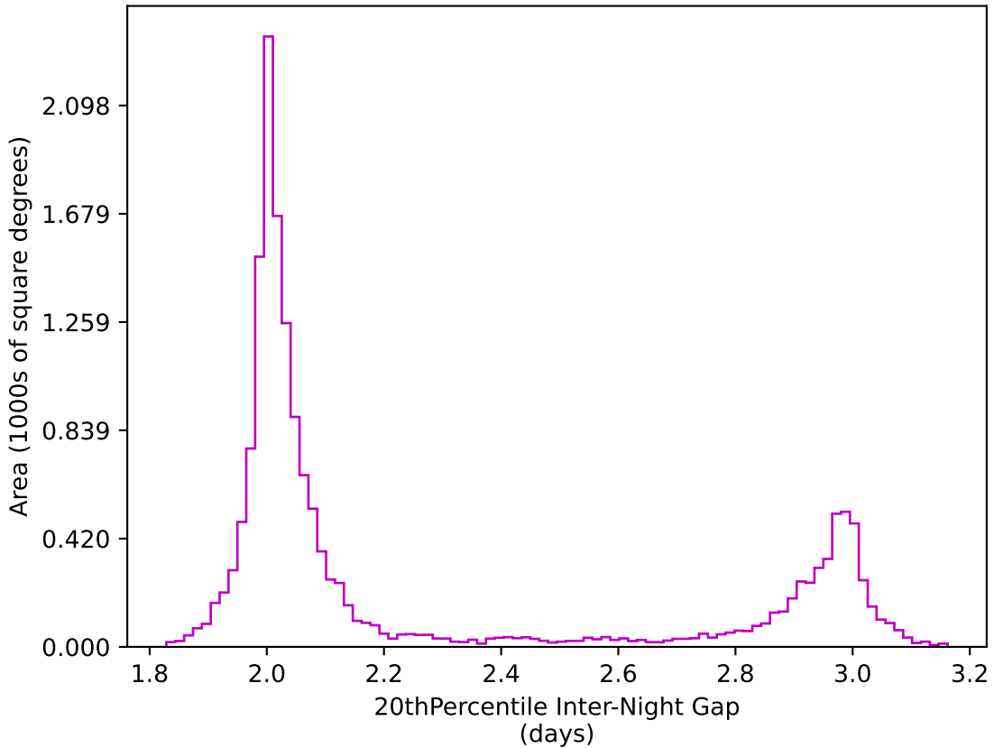
too_elab_r8_d2_griz_v3.4_10yrs WFD z band: 20thPercentile Inter-Night Gap
