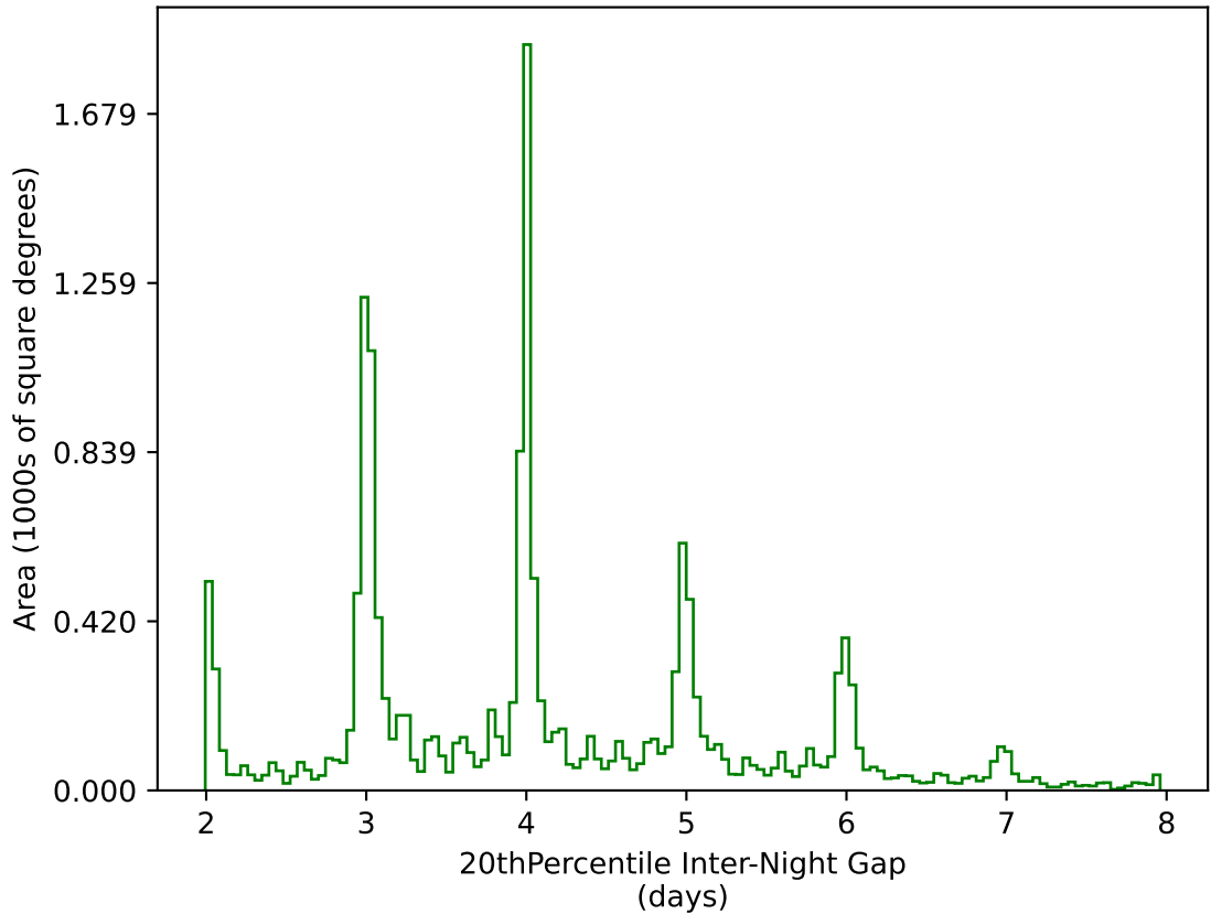
too_elab_r8_d2_griz_v3.4_10yrs WFD g band: 20thPercentile Inter-Night Gap
