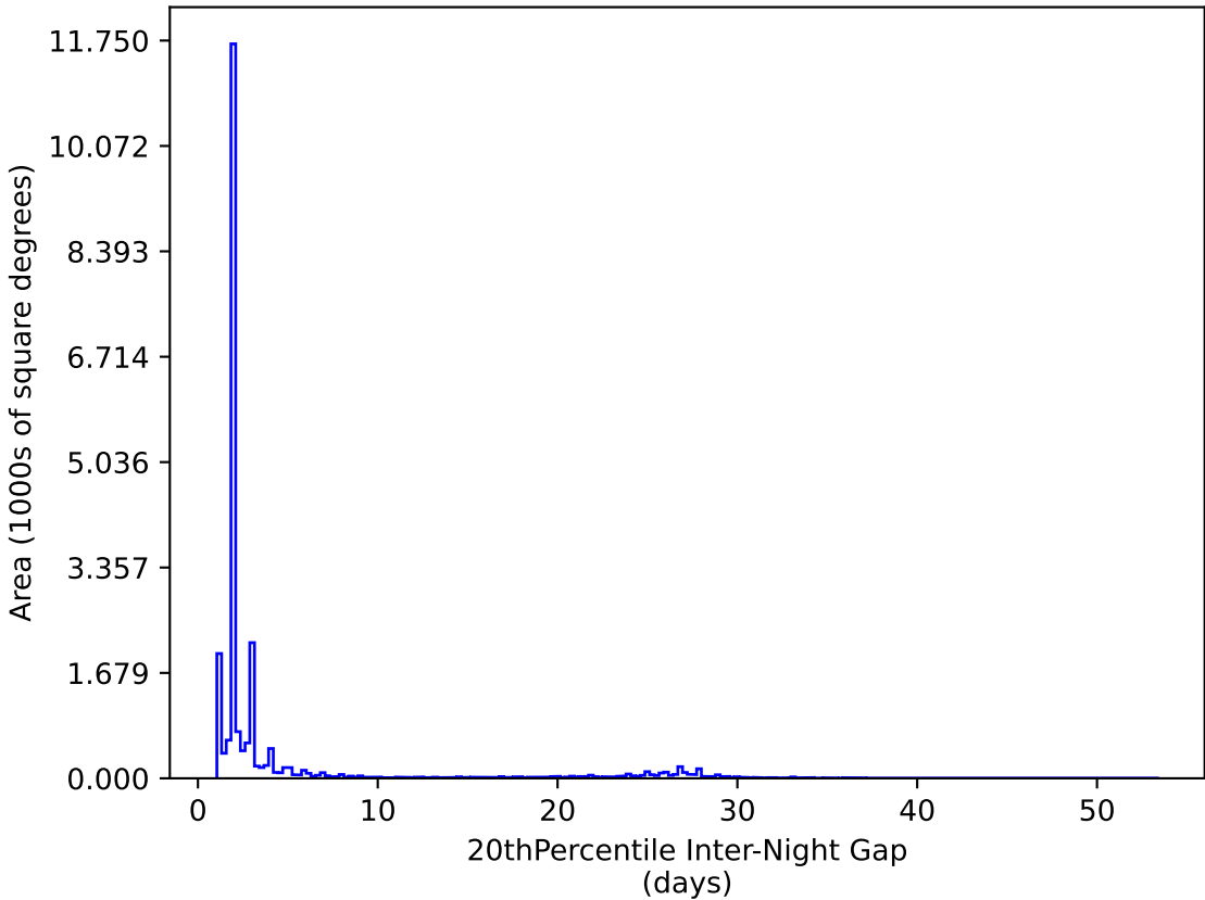
too_elab_r8_d2_griz_v3.4_10yrs All sky y band: 20thPercentile Inter-Night Gap
