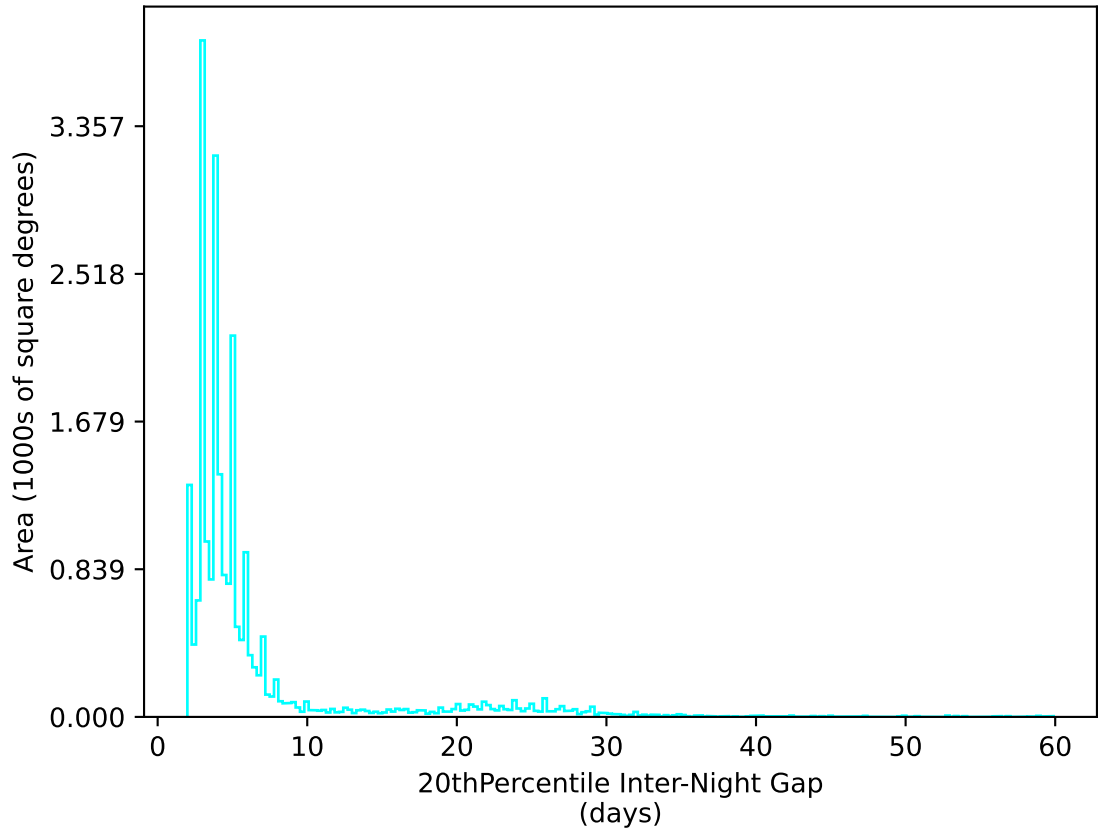
too_elab_r8_d2_griz_v3.4_10yrs All sky u band: 20thPercentile Inter-Night Gap
