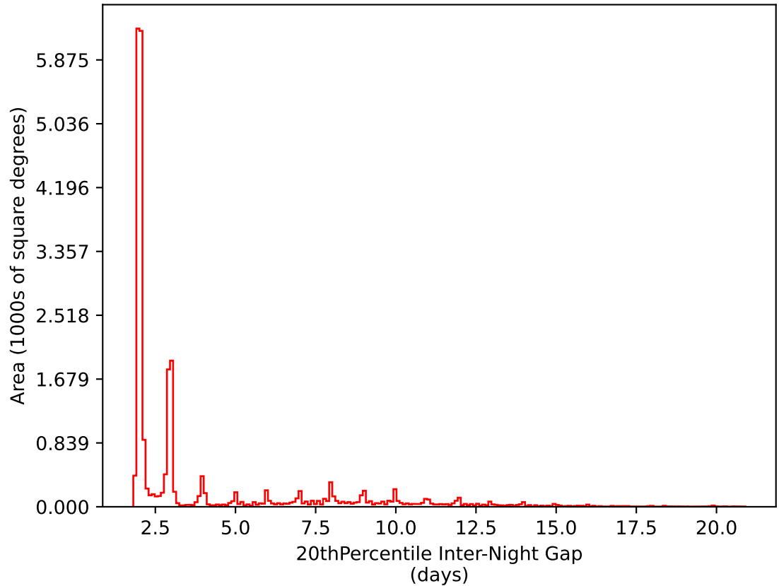
too_elab_r8_d2_griz_v3.4_10yrs All sky i band: 20thPercentile Inter-Night Gap
