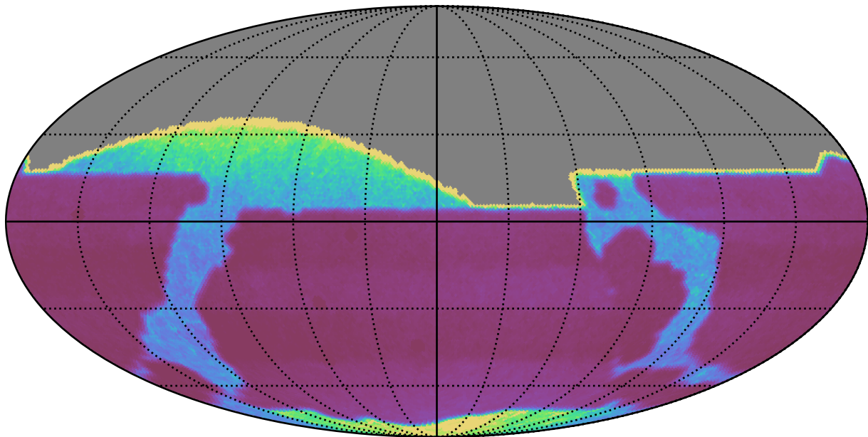
too_elab_r8_d2_griz_v3.4_10yrs : properMotion
