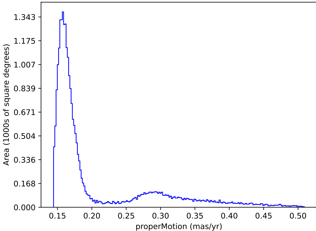
too_elab_r8_d2_griz_v3.4_10yrs : properMotion
