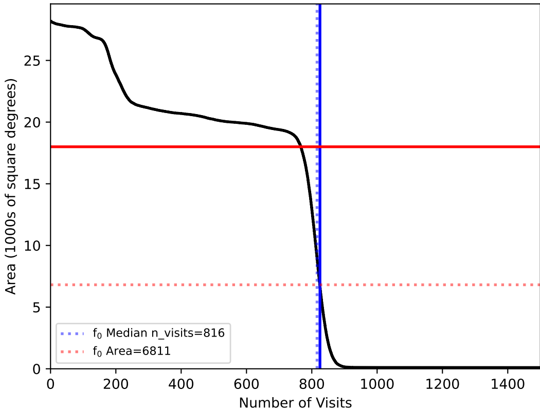
too_elab_r8_d2_griz_v3.4_10yrs : f0
