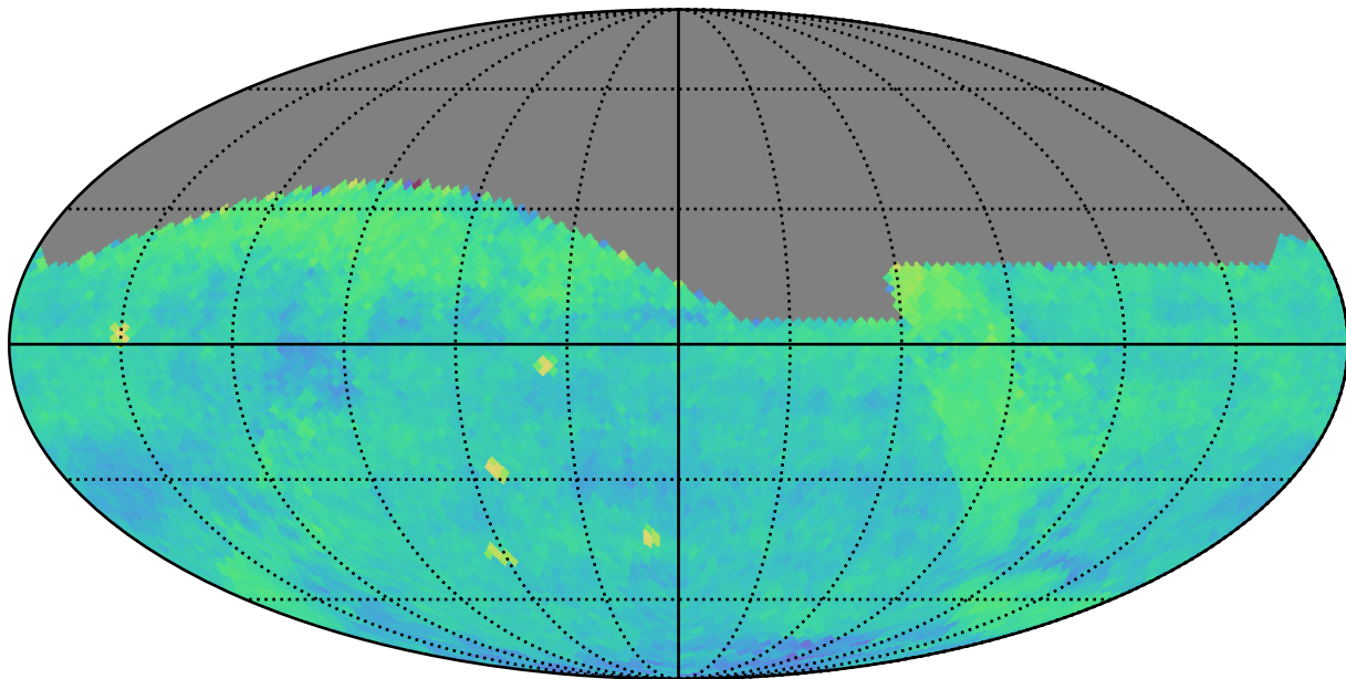
too_elab_r8_d2_griz_v3.4_10yrs (g or r or i): PairFraction
