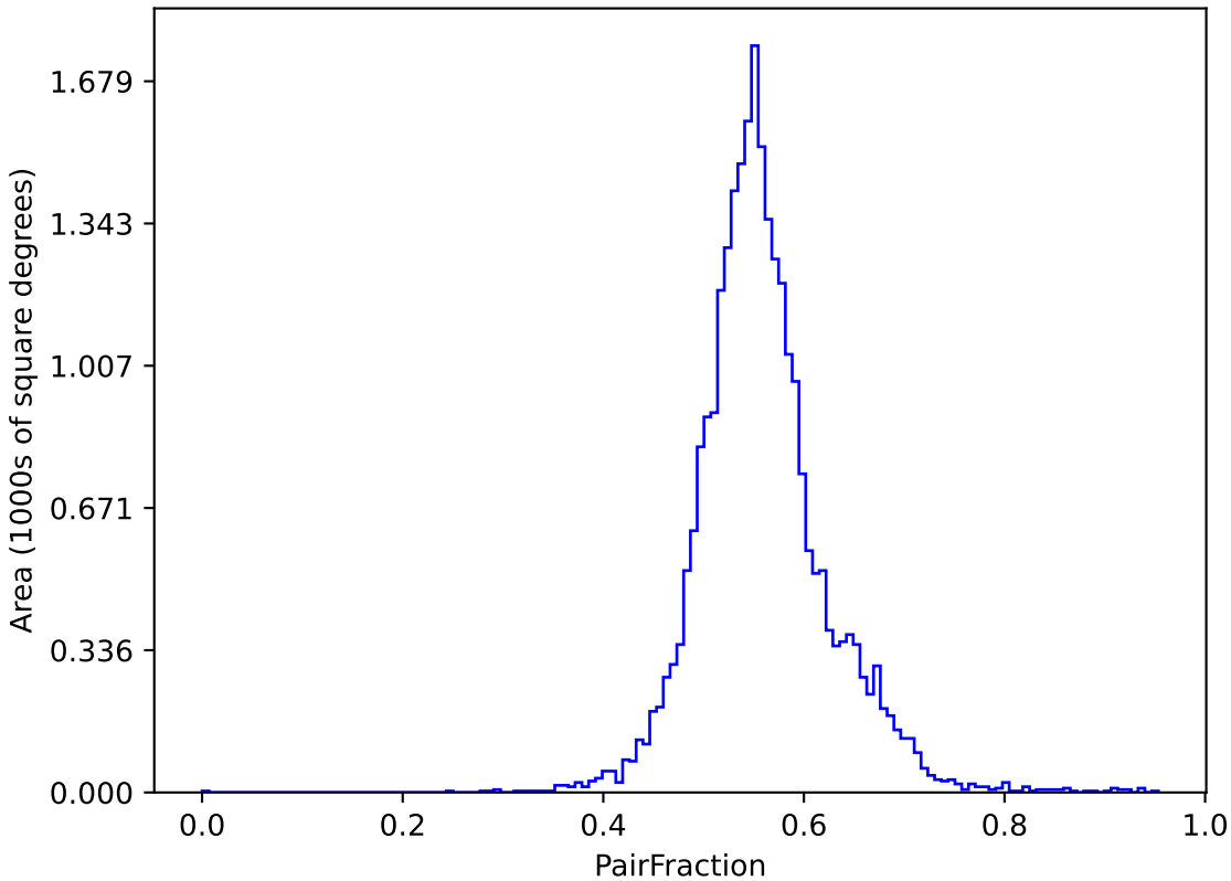
too_elab_r8_d2_griz_v3.4_10yrs (g or r or i): PairFraction
