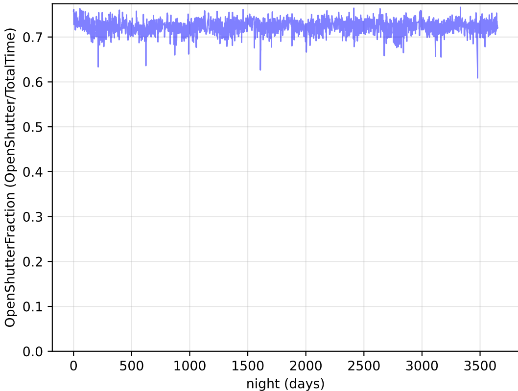
too_elab_r8_d2_griz_v3.4_10yrs : OpenShutterFraction
