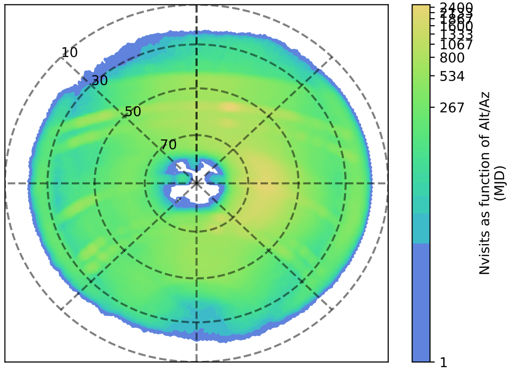
too_elab_r8_d2_griz_v3.4_10yrs z: Nvisits as function of Alt/Az
