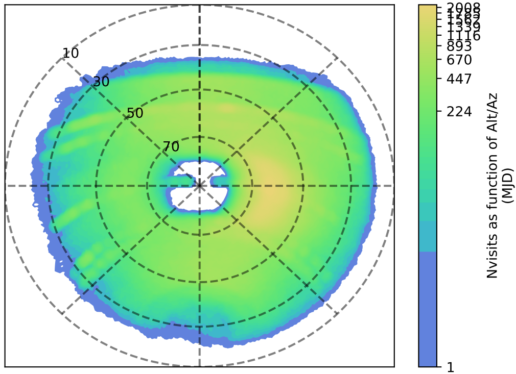
too_elab_r8_d2_griz_v3.4_10yrs y: Nvisits as function of Alt/Az
