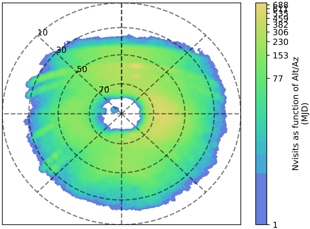
too_elab_r8_d2_griz_v3.4_10yrs u: Nvisits as function of Alt/Az
