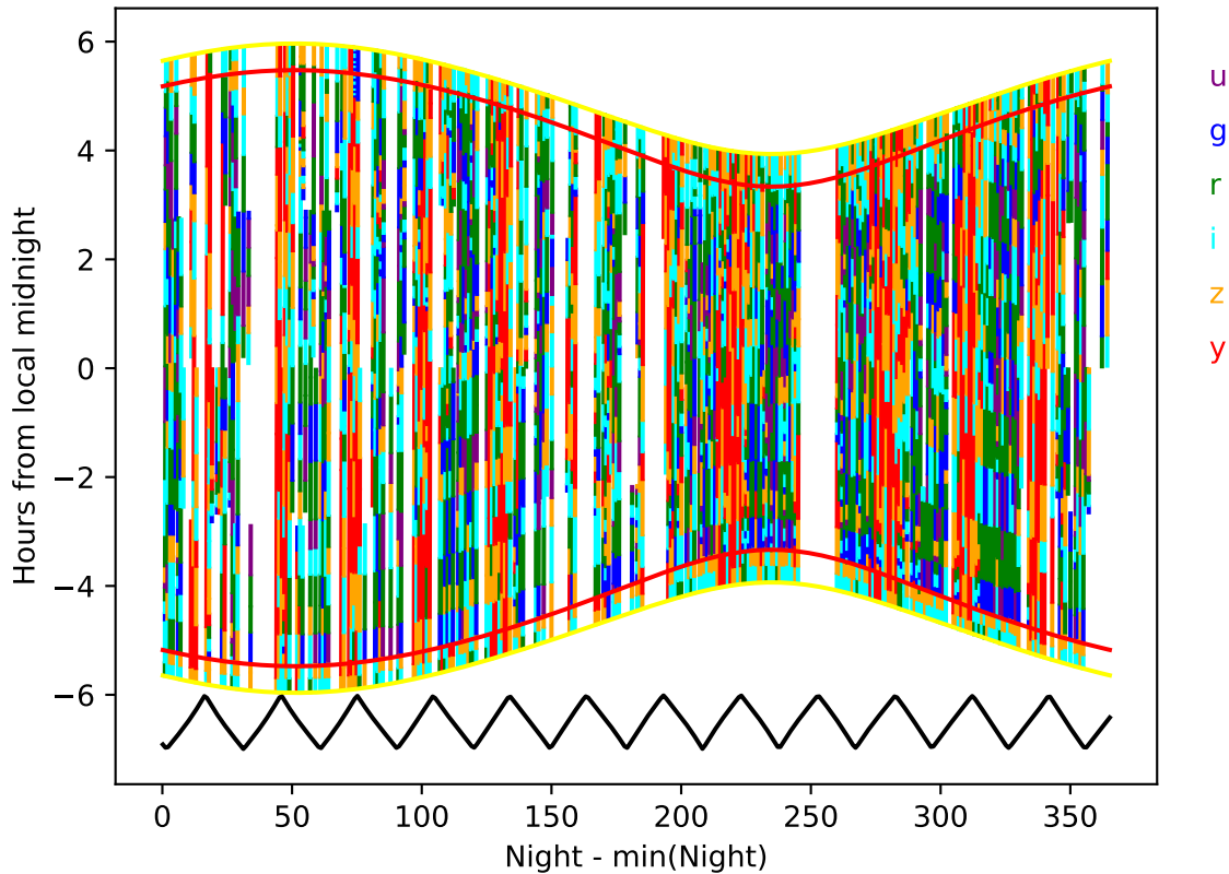
too_elab_r8_d2_griz_v3.4_10yrs year 5-6: Hourglass
