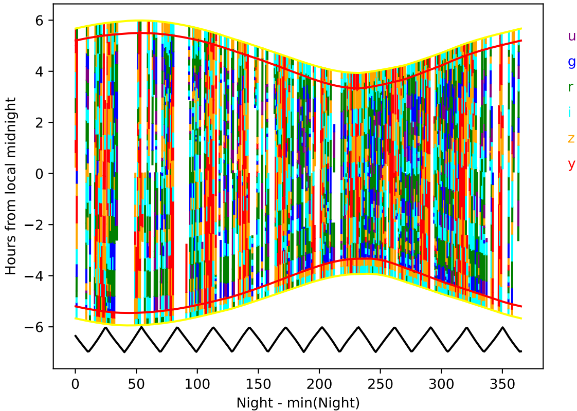
too_elab_r8_d2_griz_v3.4_10yrs year 4-5: Hourglass
